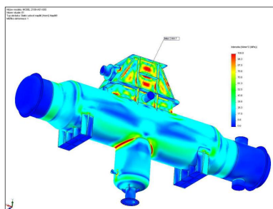
Fig. 27. Linear elastic analysis / SHELL – Stress intensity / TOP.
